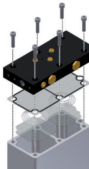
Retirer la plaque de soupapes antiretour
